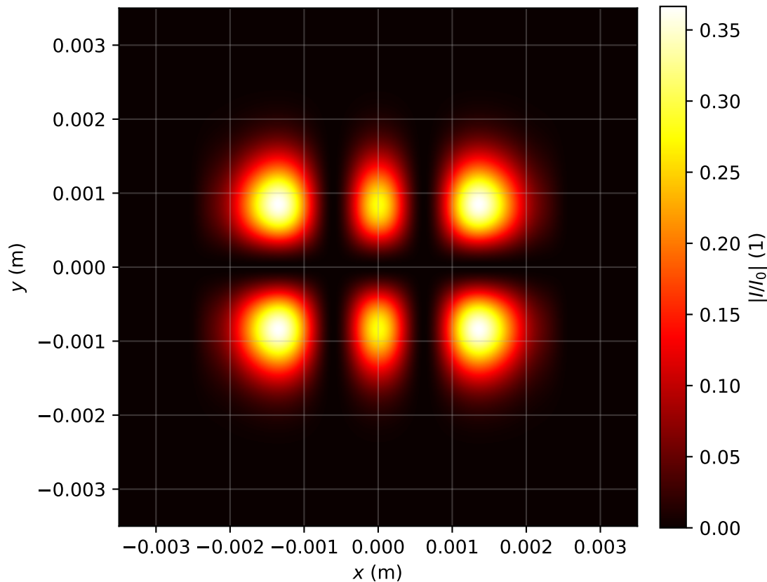
Intensity profile I(x, y, z = 2.786)/I_0 , P_{in}=0.5P_{cr} , artificial time
